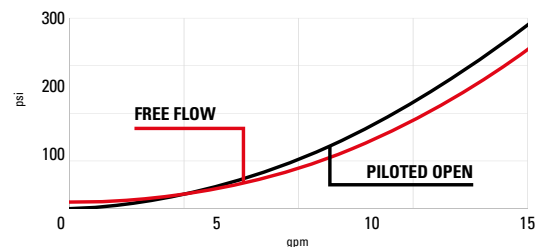
Performance curves
